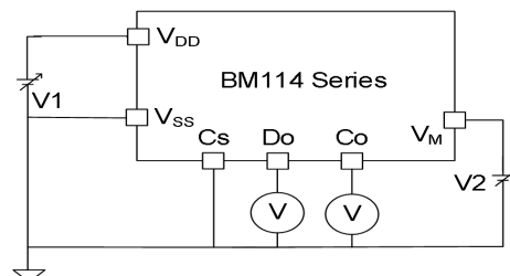
Test circuit 4
