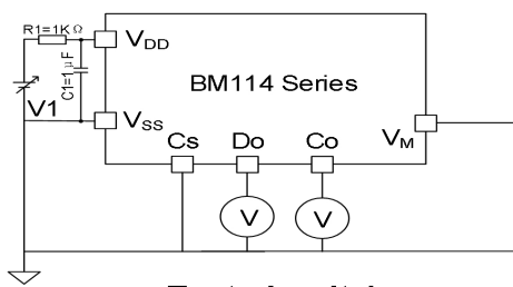
Test circuit 1
