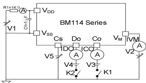
Test circuit 3
