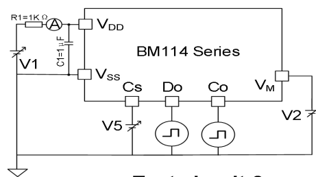
Test circuit 2
