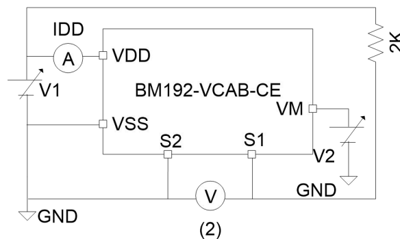
Test circuit 2
