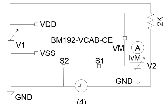
Test circuit 4
