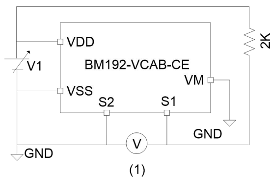
Test circuit 1
