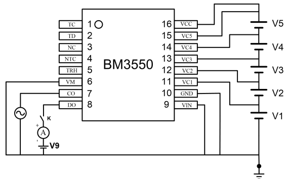
Test circuit 6
