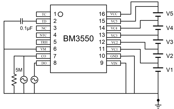
Test circuit 2
