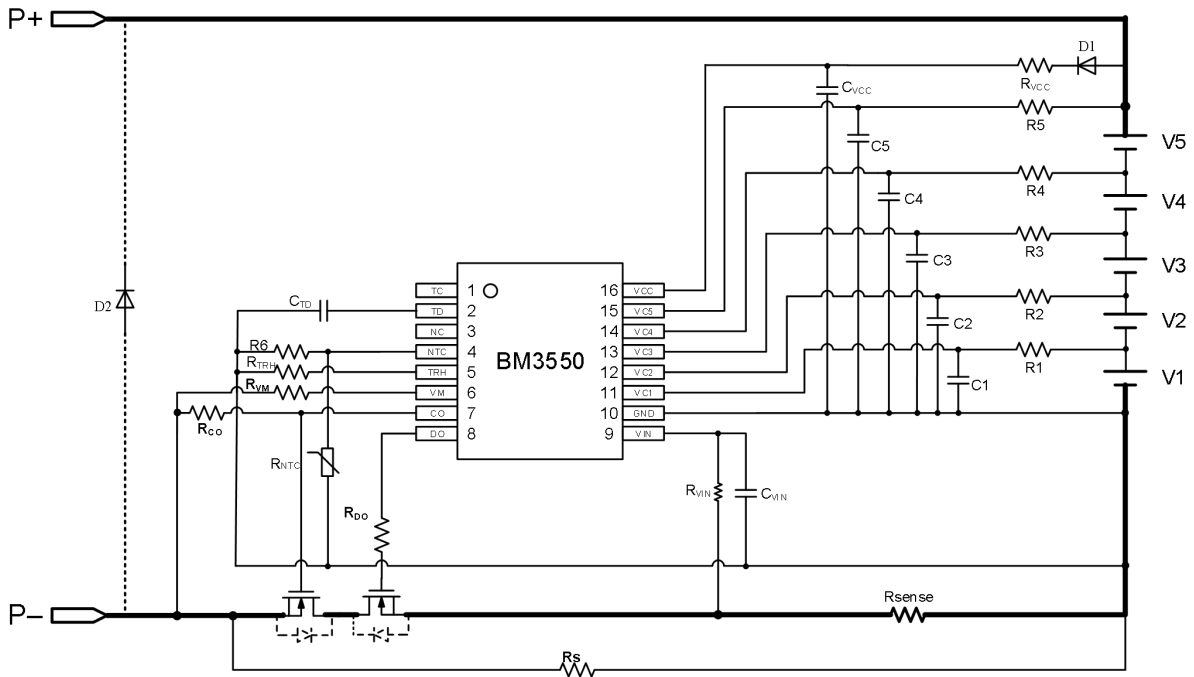
5-cell application -- charge and discharge circuits together
