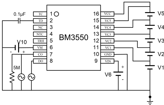
Test circuit 3
