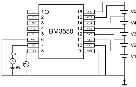
Test circuit 5
