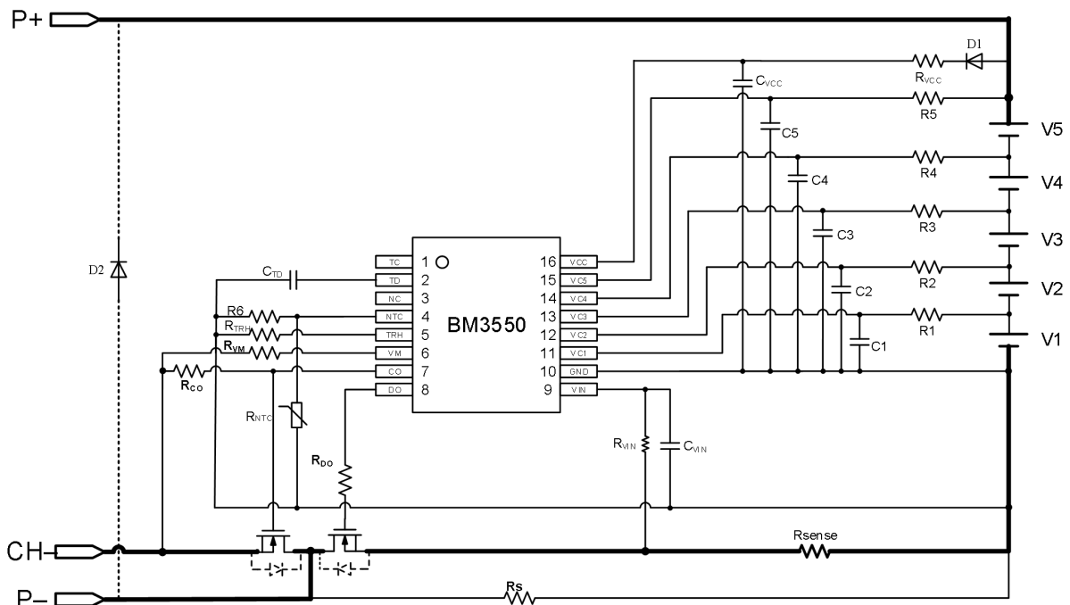
5-cell application -- charge and discharge circuits separated
