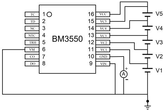
Test circuit 1
