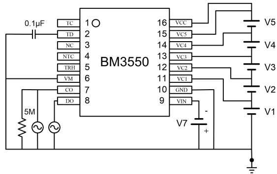
Test circuit 4
